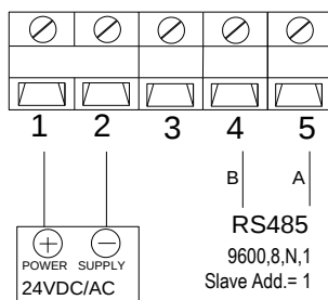
RS485/Modbus
