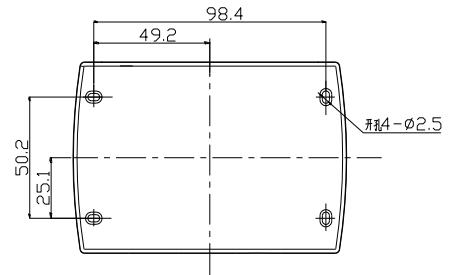
H3N/H4N 墙面安装开孔
